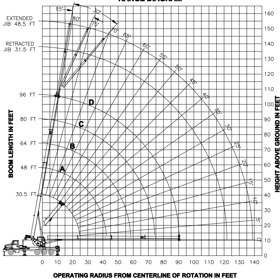
- RANGE DIAGRAM -
