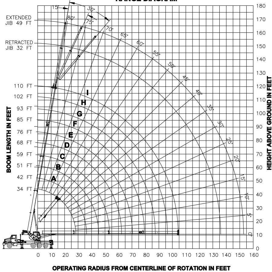
- RANGE DIAGRAM -
